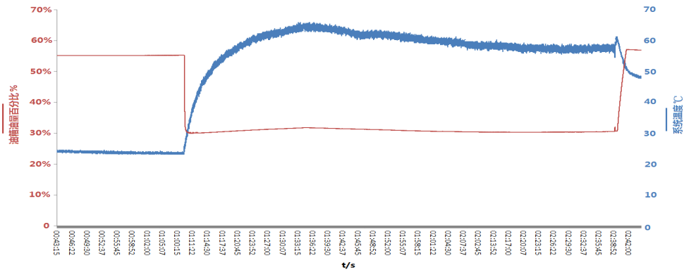
图4 机上油箱油量/油温记录曲线图(地面温度 23 °C) Fig. 4 Reservoir Fluid volume/Fluid Temperature record curve during flight(ground temp 23 °C)
