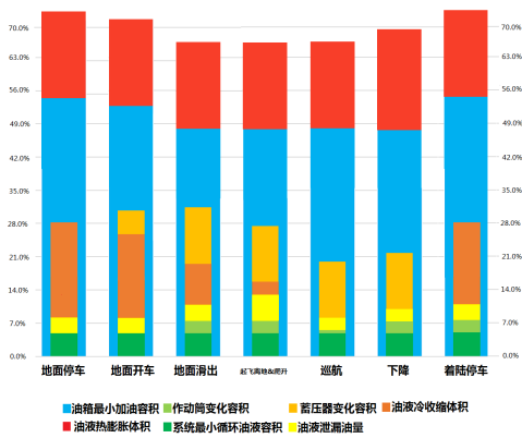
图3 飞行阶段的油箱油量变化情况分析 Fig. 3 Analysis of the change of fuel tank fuel volume during flight
