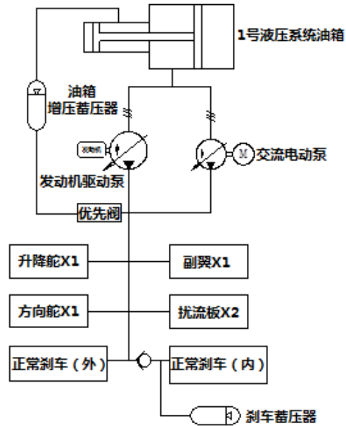
图 2 1号液压系统工作原理图 Fig. 2 Working principle diagram of No. 1 hydraulic system
