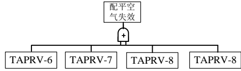
(i) 配平空气压力调节活门故障逻辑
