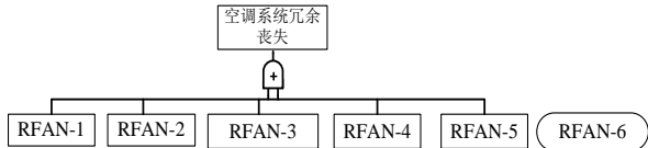
(e) 再循环风扇故障逻辑
