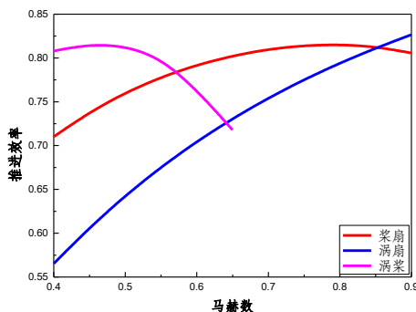
图4 推进效率随马赫数变化关系 Fig. 4 Relationship between propulsion efficiency and Mach number
