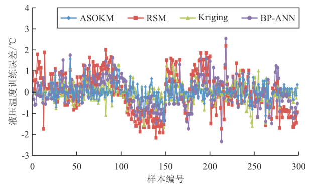
图4 液压系统训练误差结果 Fig. 4 Analysis of hydraulic system training error results
